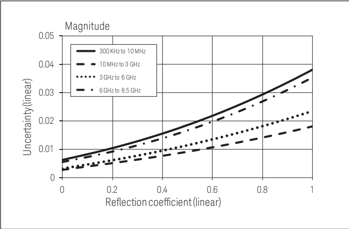
Figure 5. Reflection uncertainty (Specification)
