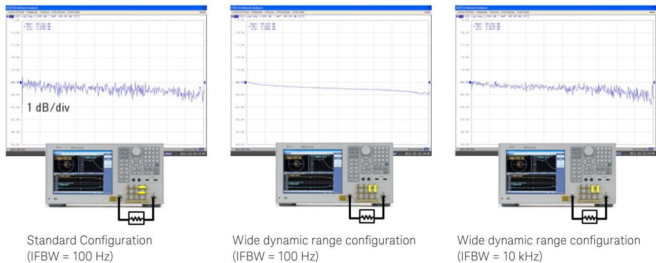
Figure 14. S21 measurement of 80 dB attenuator. Comparison between the standard configuration and wide dynamic range configuration
