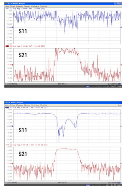
Figure 7. Accurate measurements with low signal input, Upper (power = –55 dBm with external 20 dB attenuator), Lower (power = –75 dBm with built-in attenuator)
