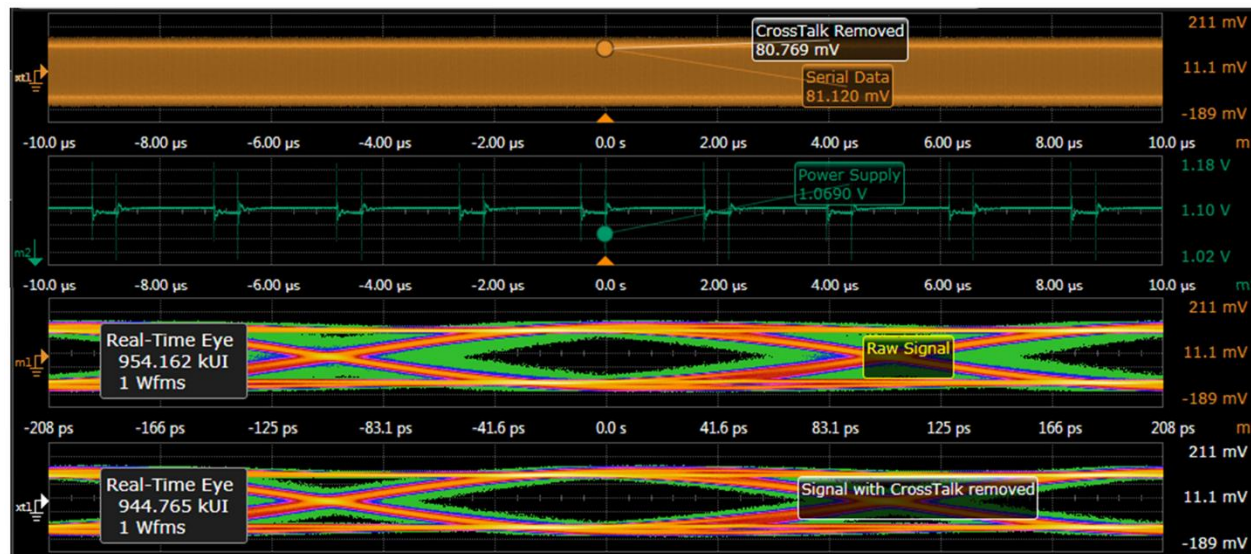
By simulating a power supply with less noise, we can realize much wider eye diagrams, leading to more robust transfer of data.
