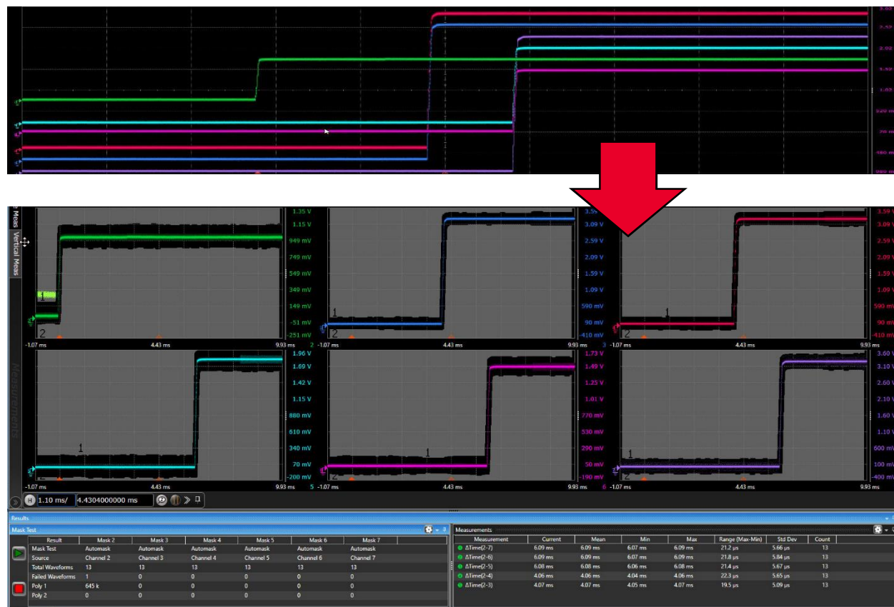
With waveforms separated into grids and independent mask tests possible on every channel, you can continuously test these six power rails over thousands of startup cycles.
